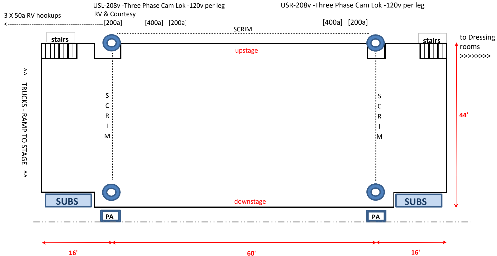
Northern Quest Outdoor Venue Stage layout & power
